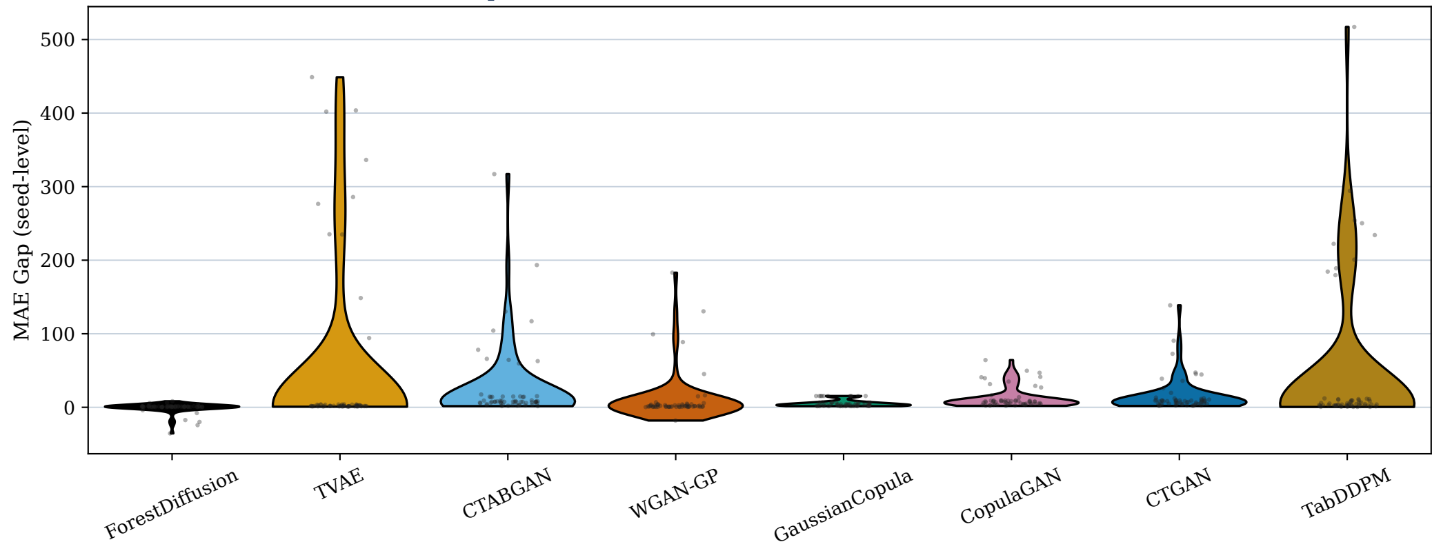
MAE Gap — seed-level distribution (n = 10 seeds × datasets)
